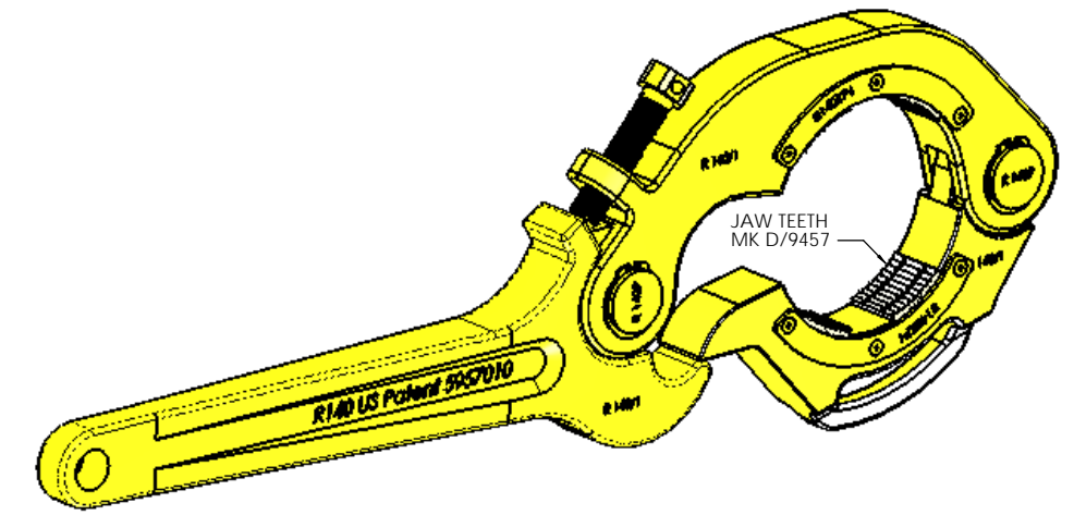
PICTORIAL VIEW
