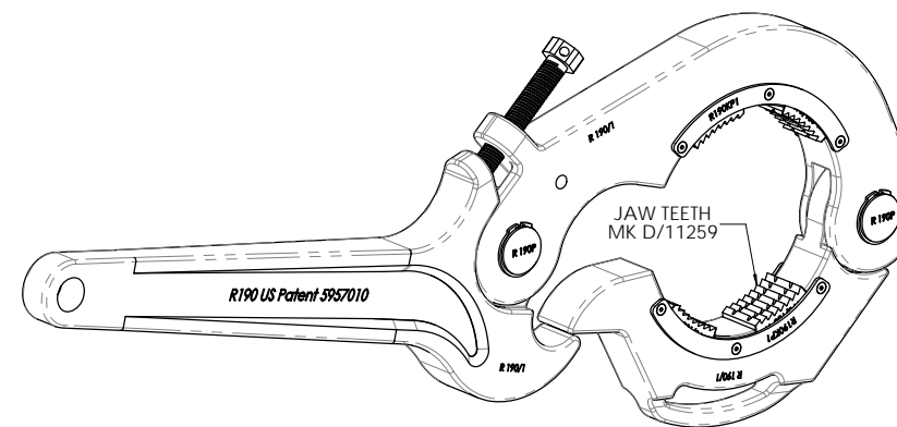
PICTORIAL VIEW Total mass with large teeth 48 Kgs.
